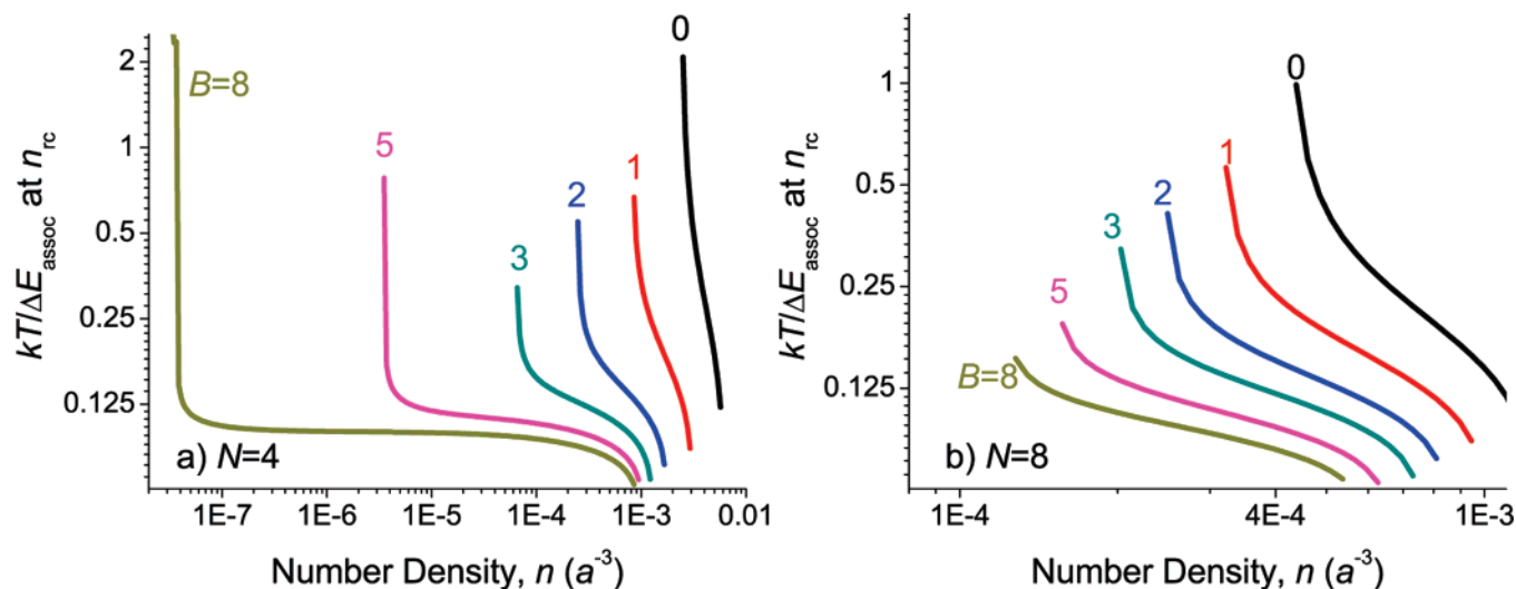
Figure 9. Numerical solutions of eq 15 for the critical kT/\Delta E_{assoc} at which ring–chain crossover occurs vs oligomer number density n at different B values and oligomer length N = 4 (a) and N = 8 (b). The area below/above each curve corresponds to the ring/chain-dominated regime.
