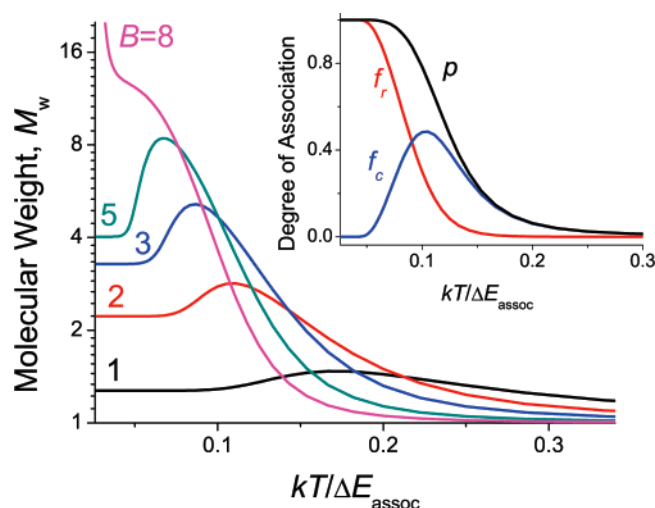
Figure 10. Numerical solutions of eq 15 for the weight-average molecular weight (in units of oligomer weight) as a function of kT/\Delta E_{\text{assoc}} for N = 4 , n = 4.8 \times 10^{-4} \text{a}^{-3} for various rigidity constants B . The inset shows the total degree of association p and the fraction of reversible bonds in rings, f_r , and chains, f_c , for B = 5 .
